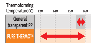
Thermoforming over a wide temperature range is possible
