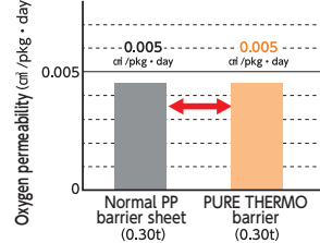
Oxygen barrier property equivalent to general PP barrier sheets
